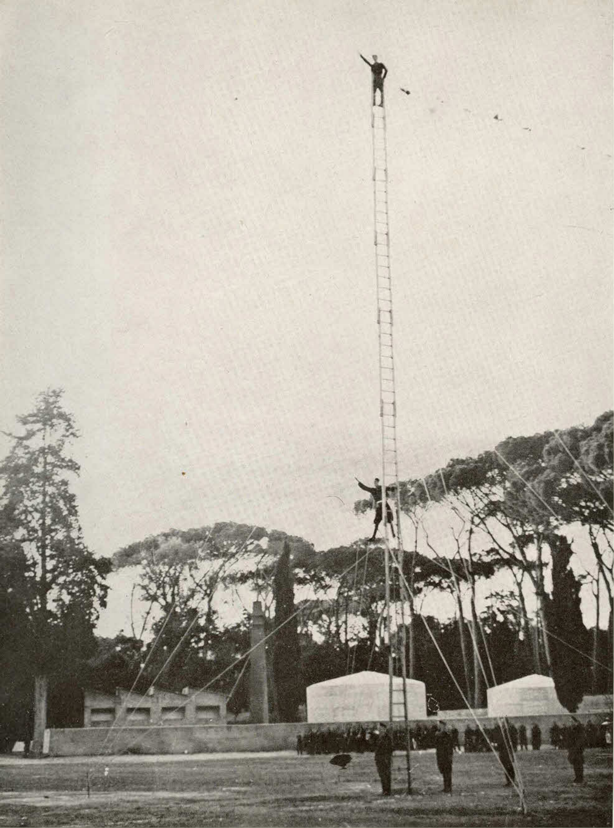
Scale romane controventate
